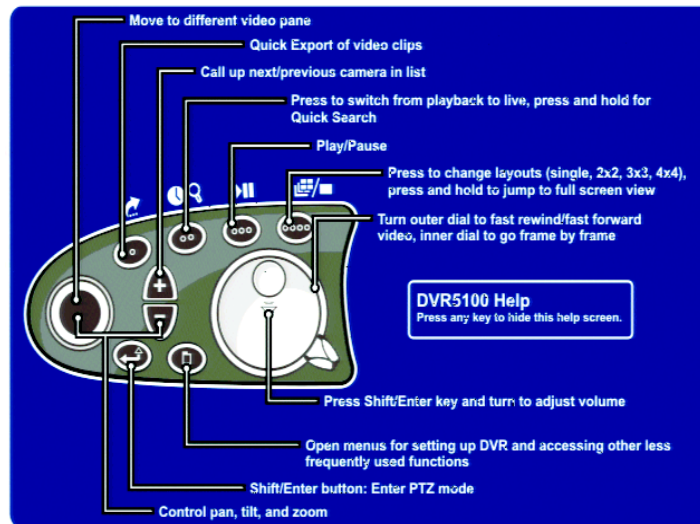
Figure 10. Control Pad Online Help Dialog Box
